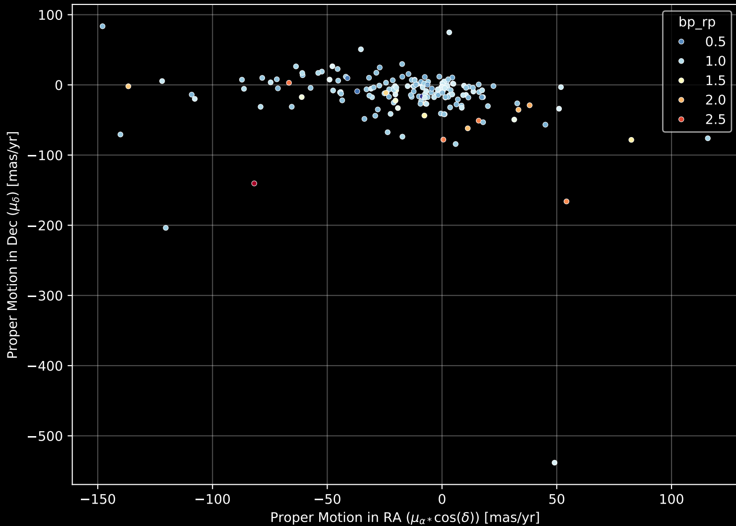
APOGEE DR17 Field: [069+83_MGA] Proper Motion Diagram (n= 175)
