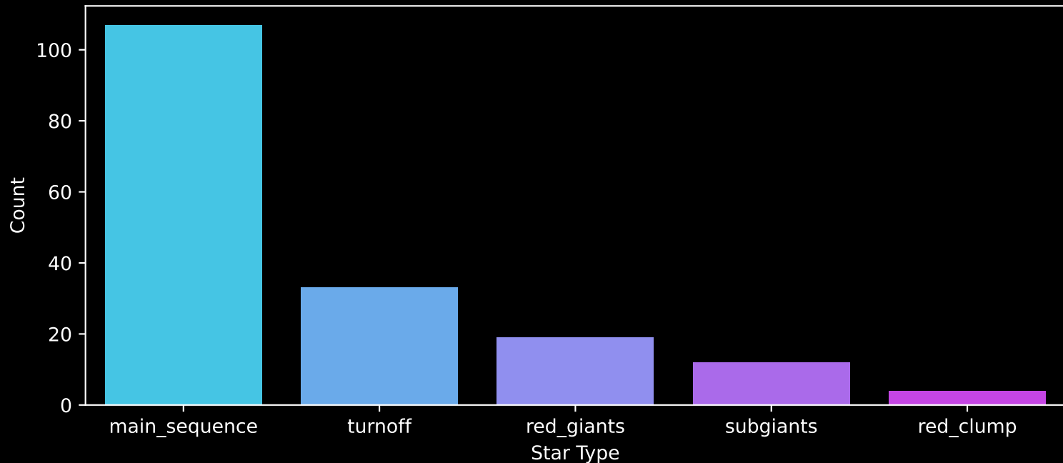
APOGEE DR17 Field: [069+83_MGA] Count plot of Star Type
