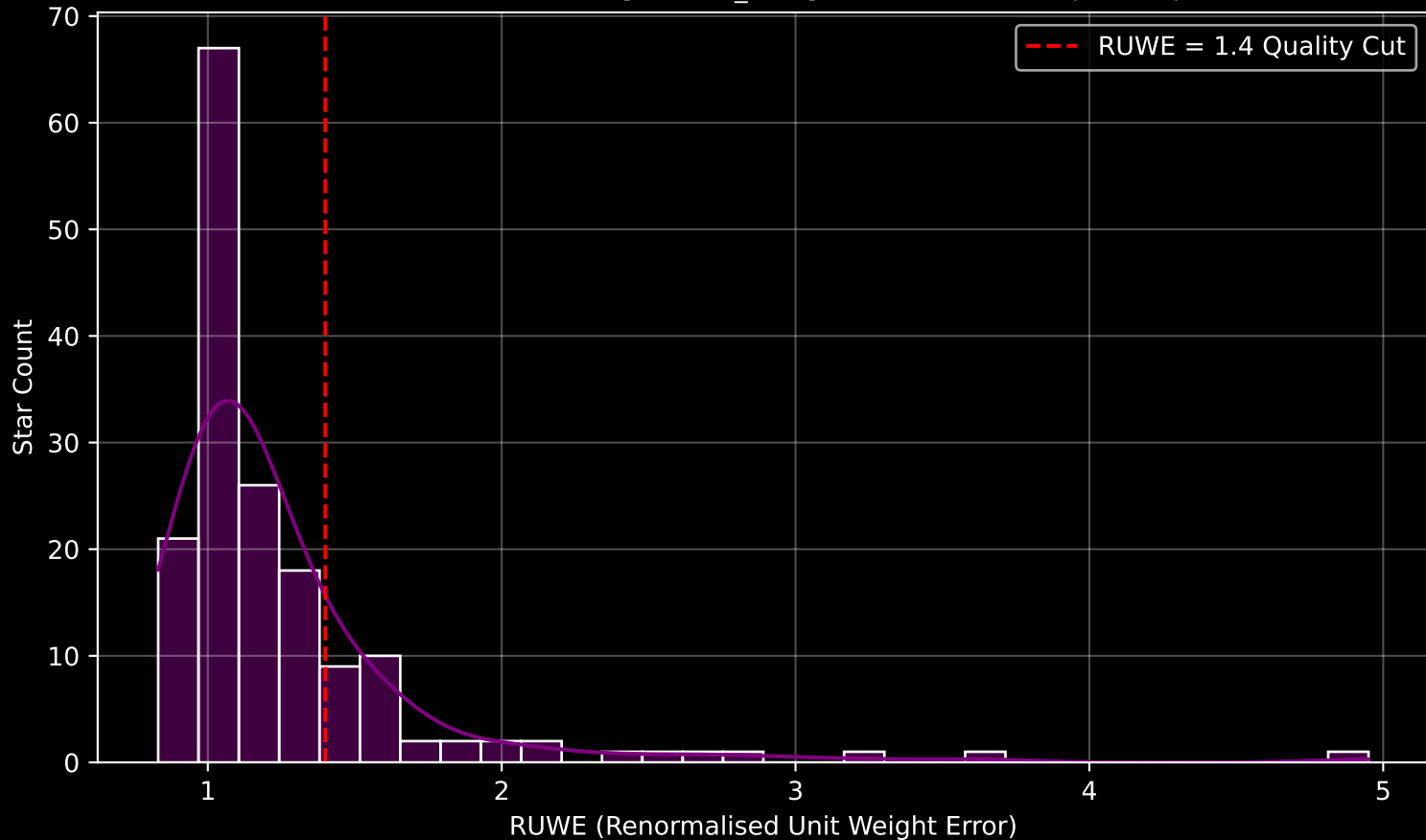
GAPOGEE DR17 Field [069+83_MGA] RUWE Distribution (n= 166)
