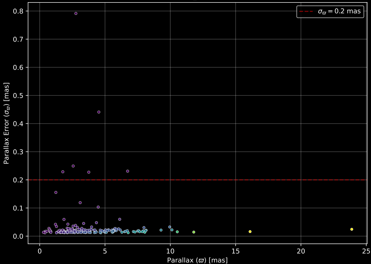
APOGEE DR17 Field: [069+83_MGA] Parallax Quality (n= 175)
