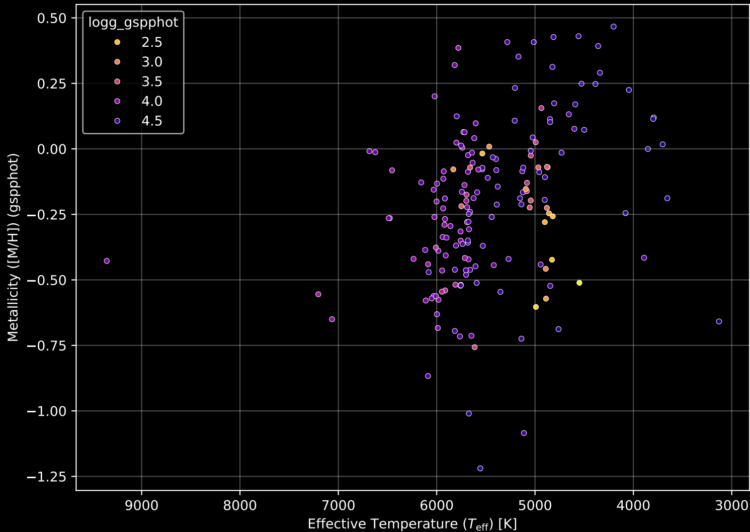
APOGEE DR17 Field: [069+83_MGA] Stellar Population Parameters (n= 175)
