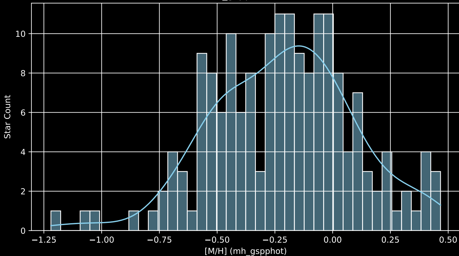
APOGEE DR17 Field: [069+83_MGA [M/H] (mh_gspphot) (n= 175)
